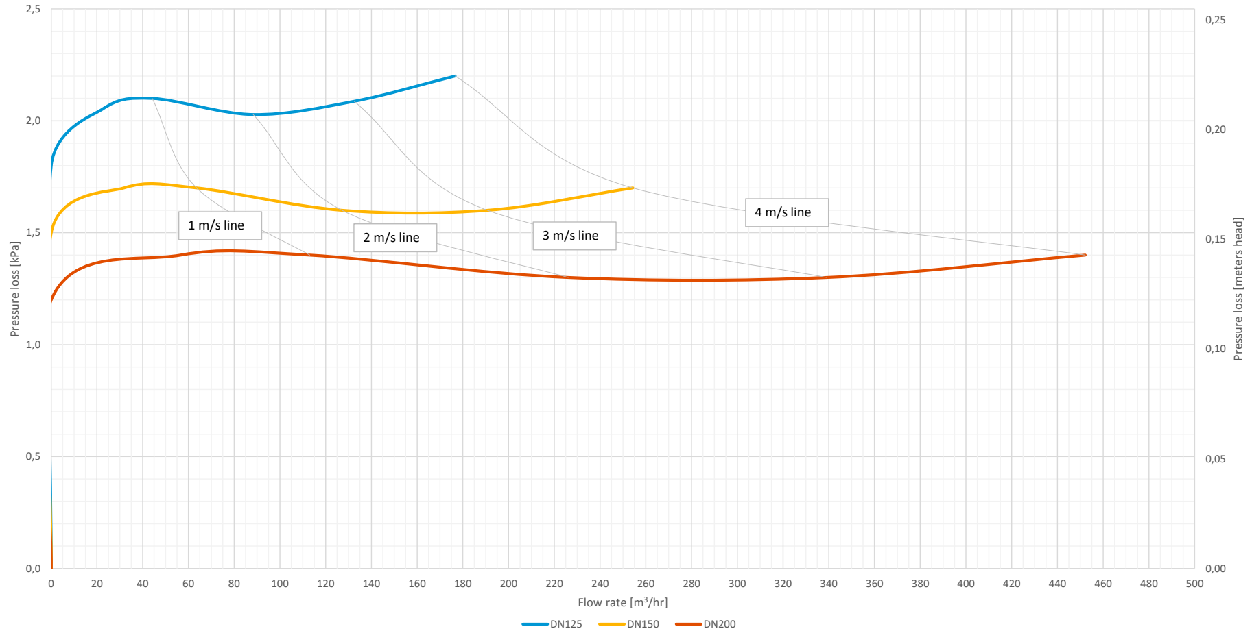
Pressure loss - Series 41 - Weight Out - DN125, DN150 and DN200
